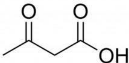
Acetoacetic acid
