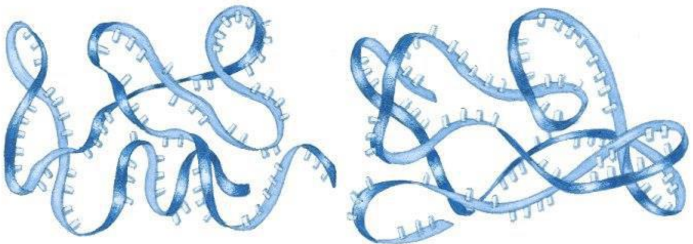
Separated strands of DNA in random coils
