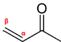
Enone
