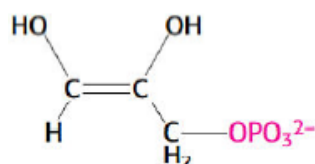
Enediol intermediate
