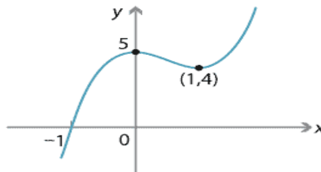
Graph of f(x) = 2x^3 - 3x^2 + 5 .
