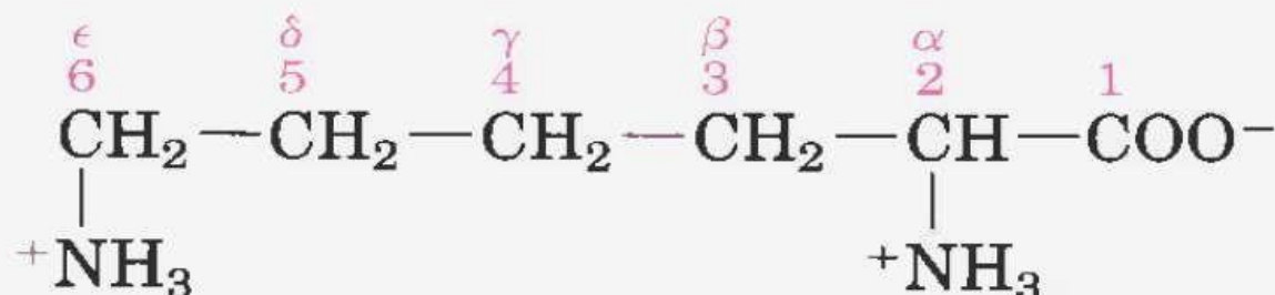
Lysine
