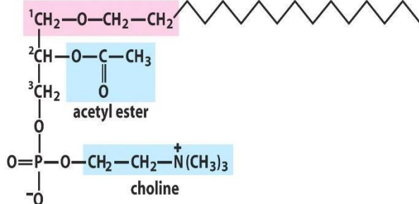
Platelet-activating factor
