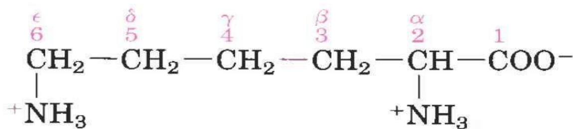
Lysine
