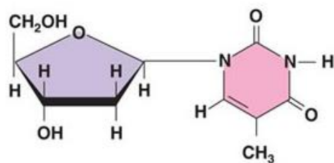
Thymine nucleoside
