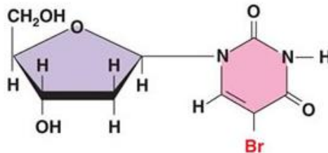
5-Bromouracil nucleoside
