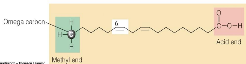
Linoleic acid, an omega-6 fatty acid
