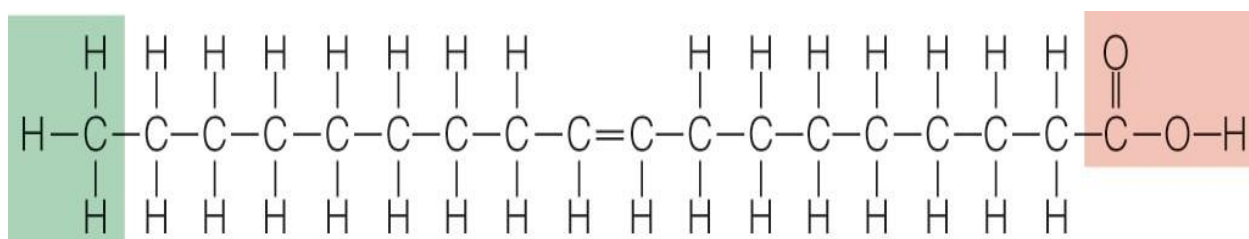
Oleic acid – 18-carbon, monounsaturated
