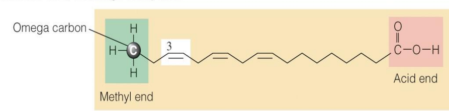
Linolenic acid, an omega-3 fatty acid
