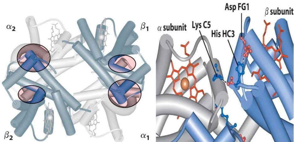
Left: Hemoglobin Structure Showing Inter chain Contact Points Right : One of the contact points magnified, showing Lys, Asp and His.
