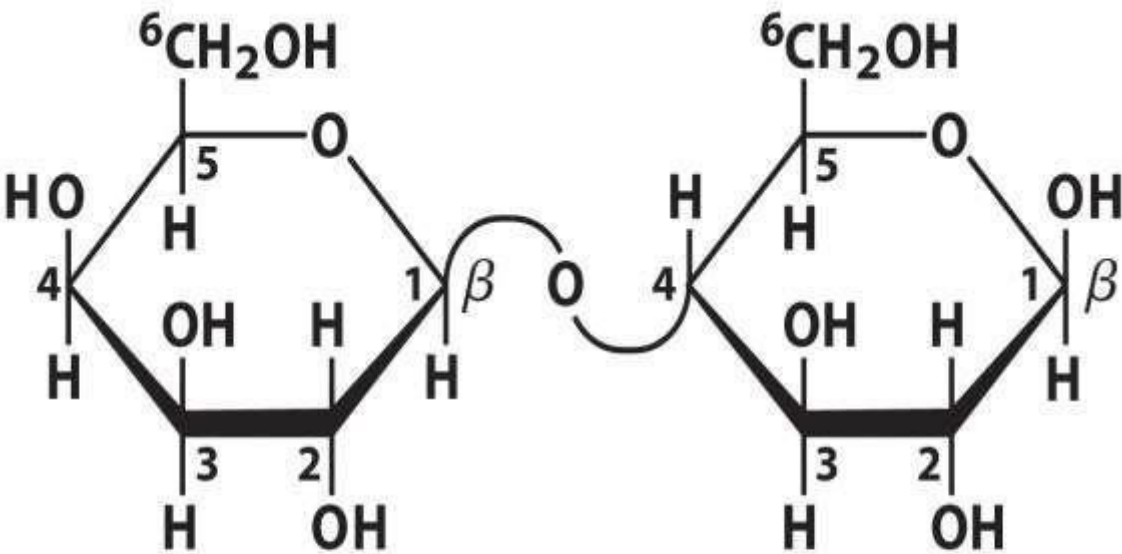
Lactose ( \beta form) \beta -D-galactopyranosyl-(1 \rightarrow 4)- \beta -D-glucopyranose Gal( \beta 1 \rightarrow 4)Glc
