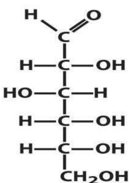
D-Glucose, an aldohexose
