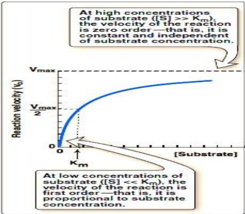
Reaction Orders with Respect to Substrate Concentration
