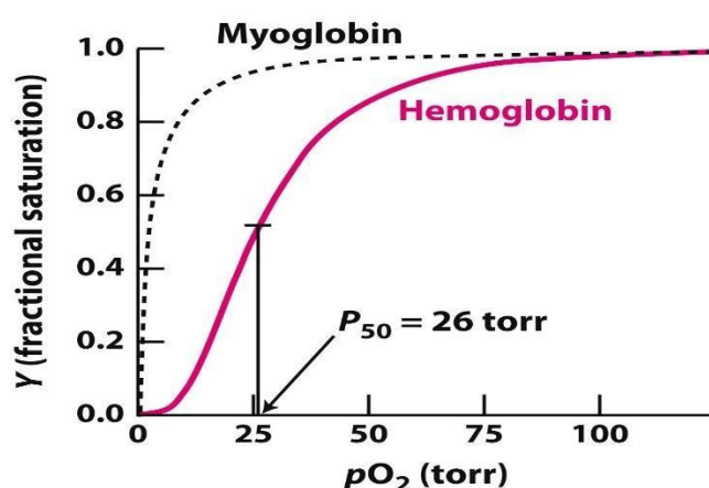
Figure 7.8 Biochemistry, Seventh Edition © 2012 W. H. Freeman and Company
