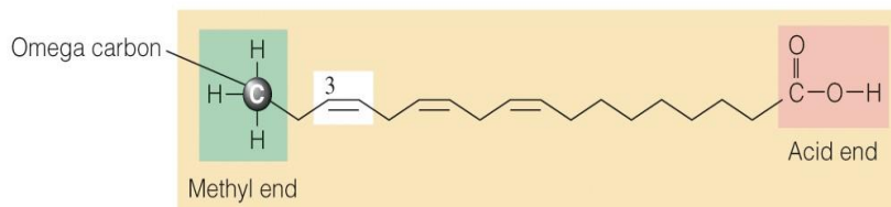
Linolenic acid, an omega-3 fatty acid
