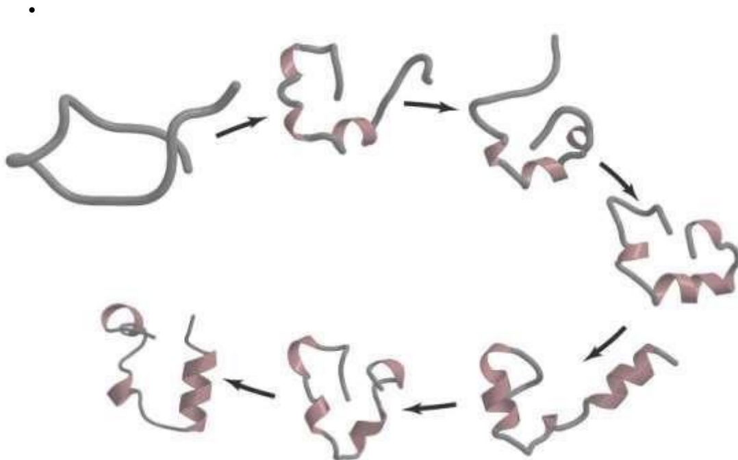
Computer simulated Protein folding showing local assembly followed by global protein folding .
