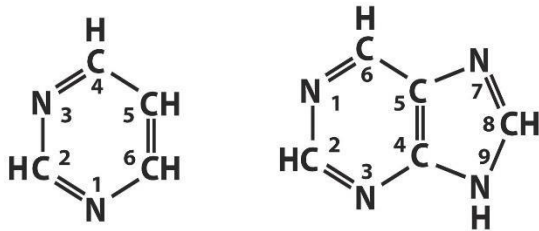
Pyrimidine
