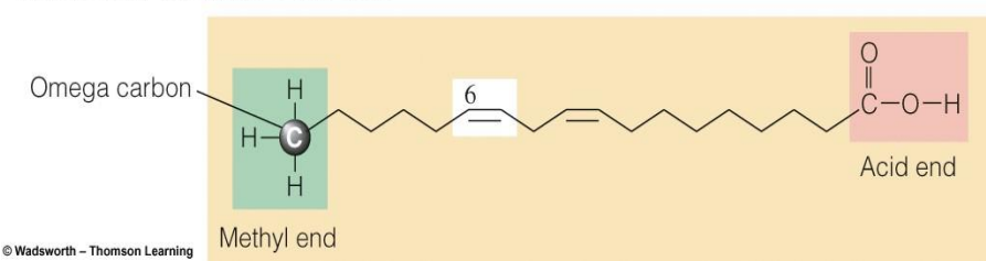
Linoleic acid, an omega-6 fatty acid
