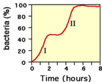
Figure 2: Monod's "bi-phasic" growth curve
