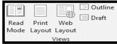
Figure 198: Views group
