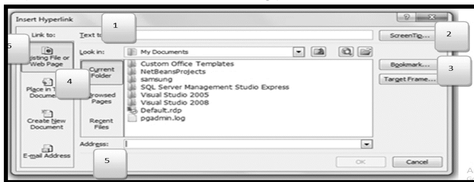
Figure 173: Adding Hyperlink
