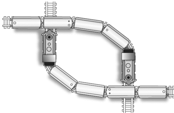
Figure 58: Deadlock Situation
