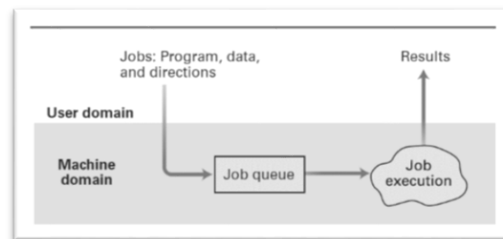
Figure 50: Batch Processing
