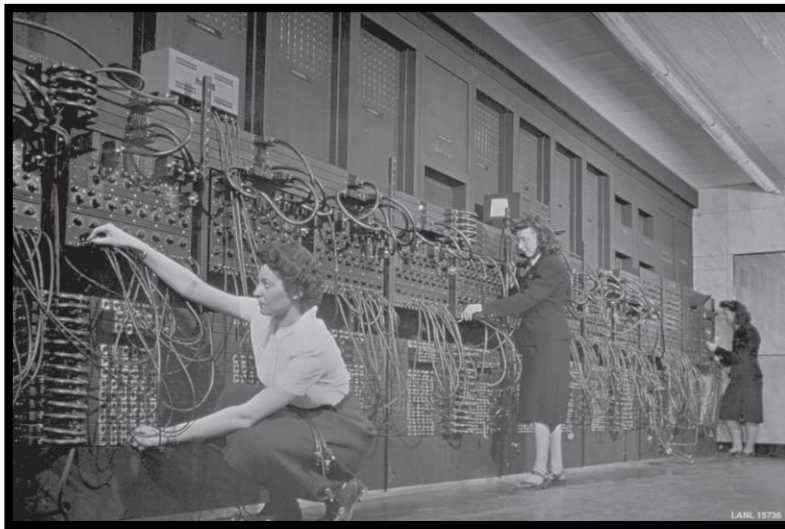
Figure 14: ENIAC
