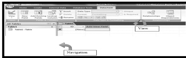
Figure 230: Blank Database
