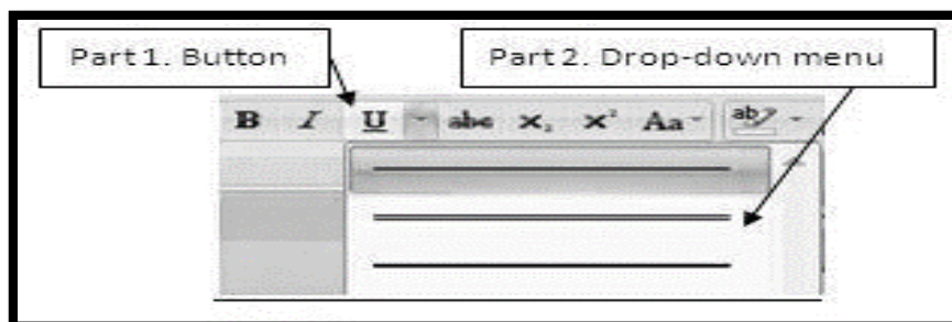
Figure 136: Underline Panel
