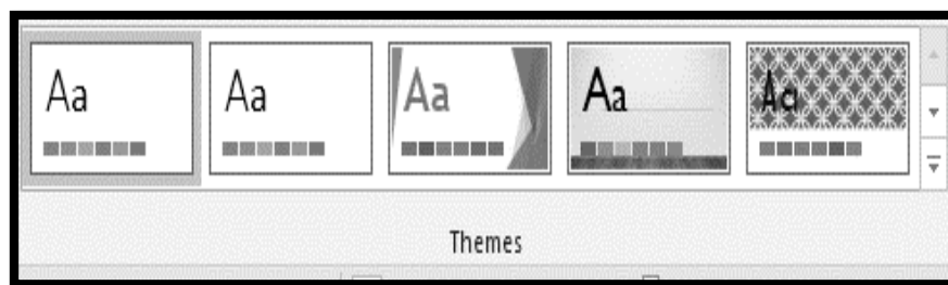
Figure 204: Themes group
