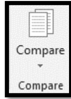
Figure 196: Compare group
