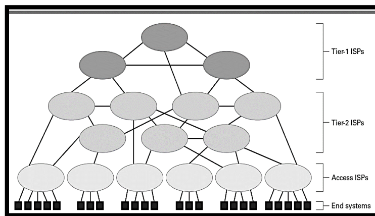
Figure 65: Internet composition
