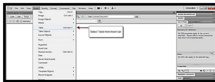
Figure 251: Insert Table
