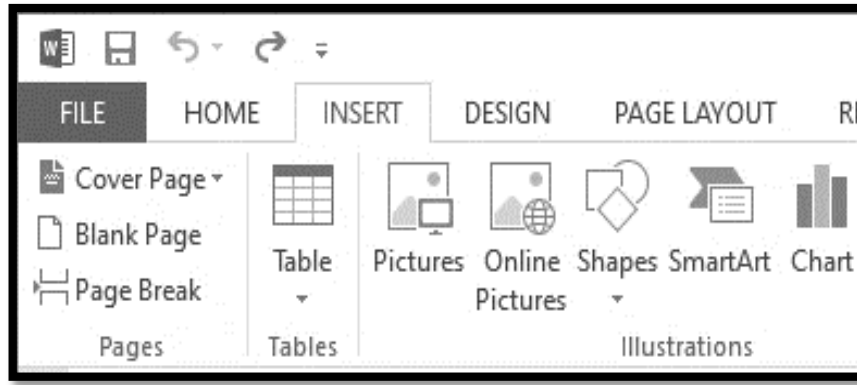
Figure 164: Illustrations
