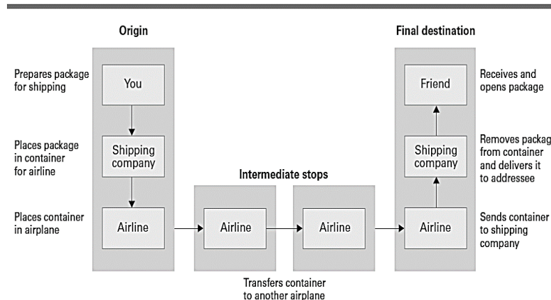
Figure 73: Package-shipping example
