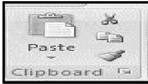
Figure 141: Clipboard Group
