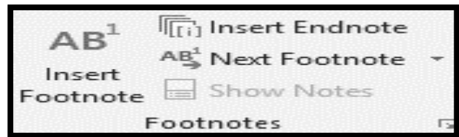
Figure 190: Footnotes Group
