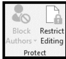
Figure 197: Protect group
