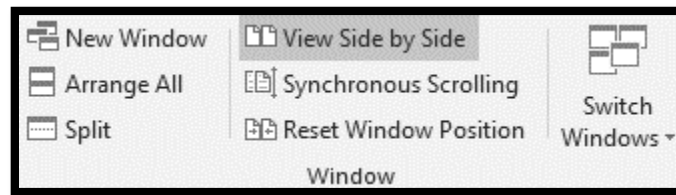
Figure 201: Windows group
