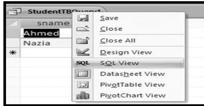
Figure 239: SQL View
