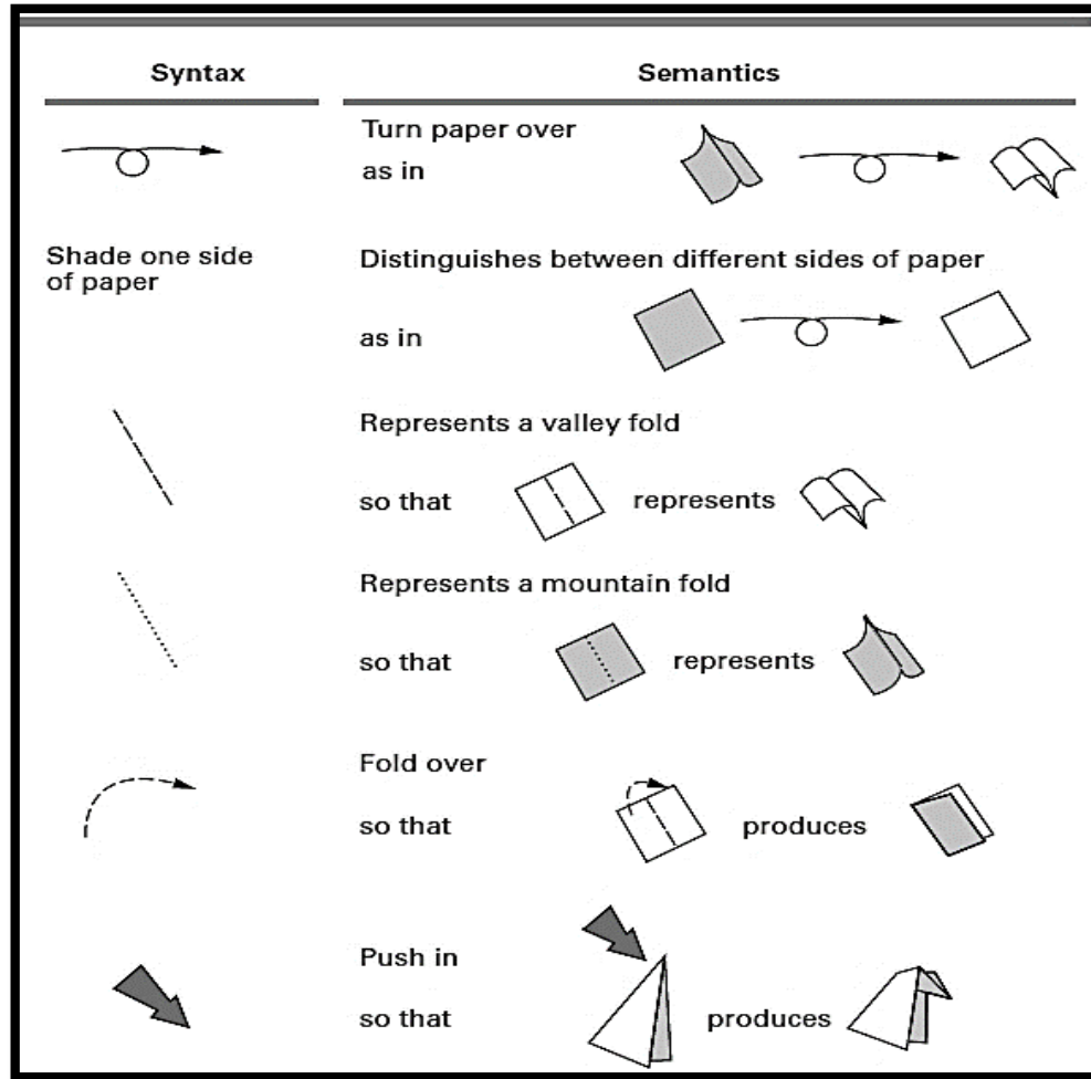
Figure 79: Origami primitives
