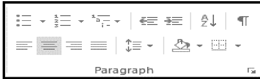
Figure 151: Paragraph Group
