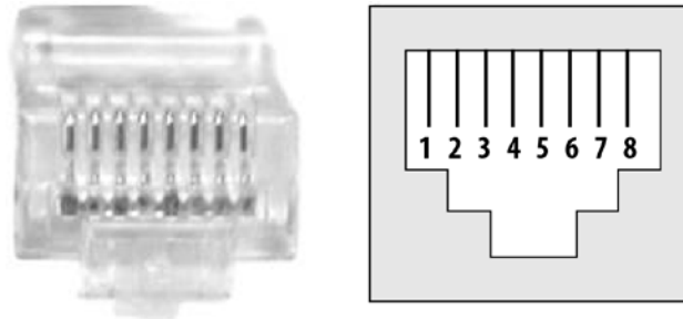
Figure 13.3: Typical Networking connector (RJ 45)
