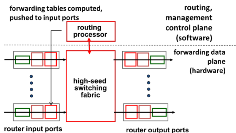
Figure 53.1: Router Hardware Architecture
