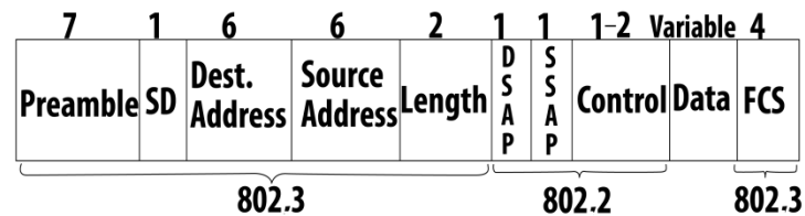
Figure 19.1: IEEE Ethernet Headers and Trailers
