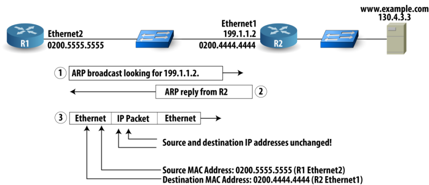
Figure 51.2: Encapsulation
