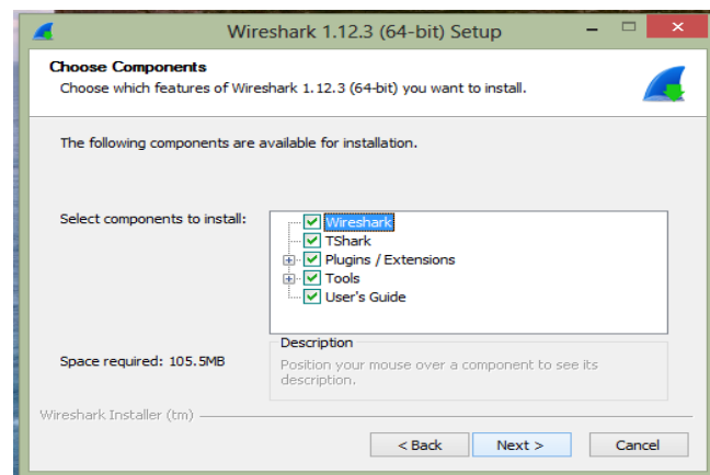
Figure 80.2: choose components
