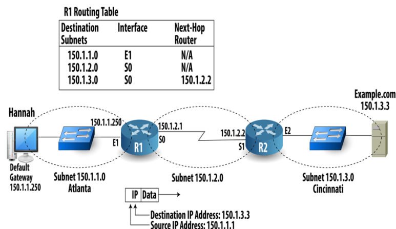
Figure 65.2: WAN data link framing
