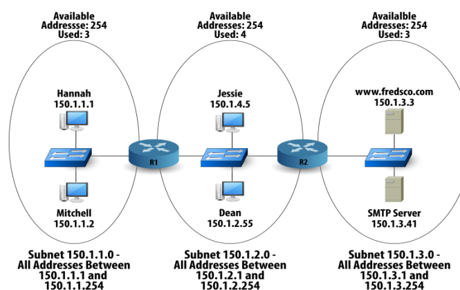
Figure 42.2: IP Subnetting
