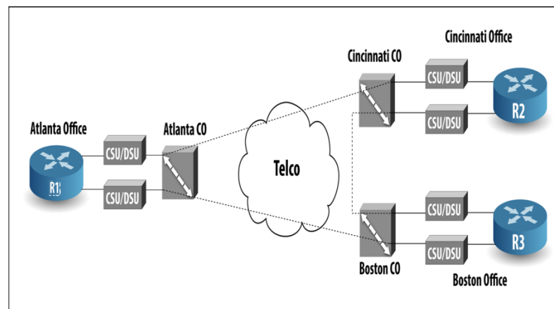
Figure 69.1: Three Leased Lines to Connect Three Routers
