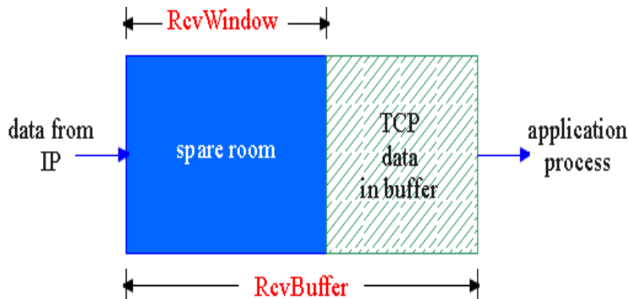
Figure 34.1 Receive Window
