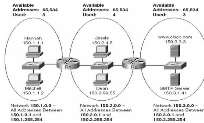
Figure 42.1: IP Subnetting
