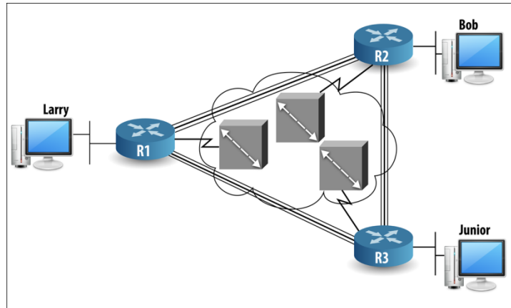
Figure 68.3: Frame Relay Full Mesh
