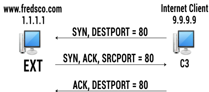
Figure 79.2: TCP Connections and Well-Known Ports
