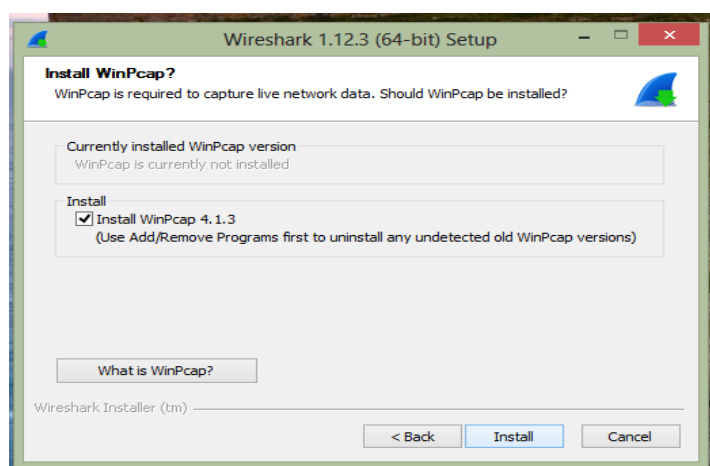
Figure 80.4: Installing WinPcap
