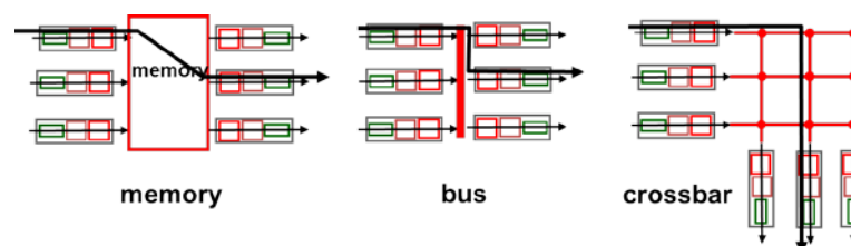
Figure 53.3: Switching fabrics
