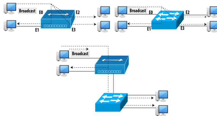
Figure 25.1: Three Broadcast Domains: A Hub, a Switch, and a Hub and Switch
