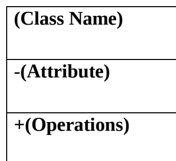
Normal Form
