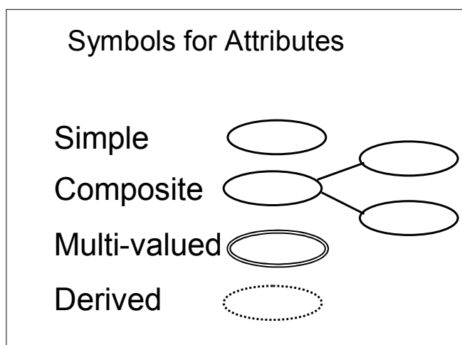
Figure 3.8 Symbols used for different types of attributes in ER diagram.
