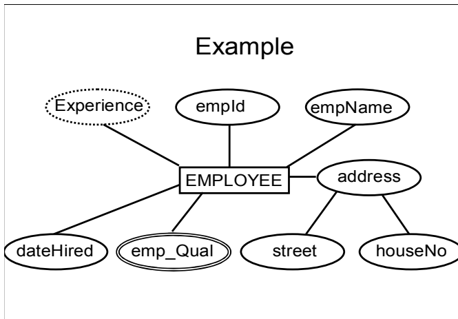
Figure 4-1: Example of an entity type with attributes of different types
