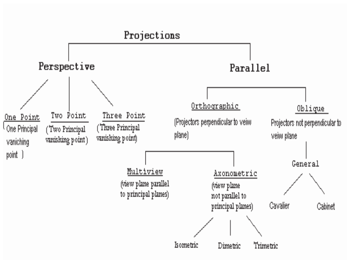
Taxonomy of Projection
