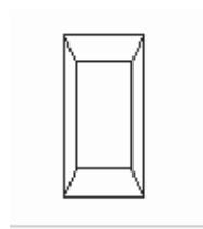
Figure 3: Transformed Cube
