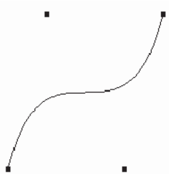
Figure 1 : Bézier Curve
