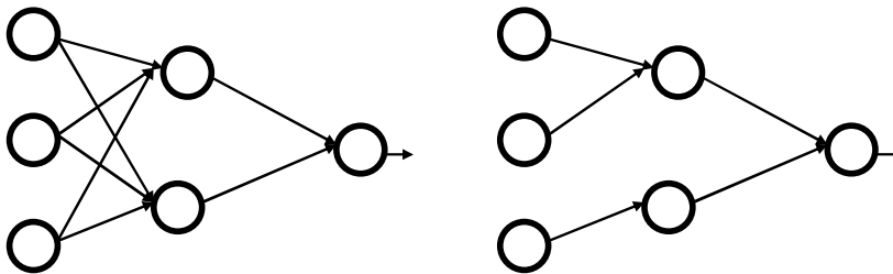
Fully connected
