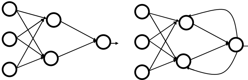
Feed forward
