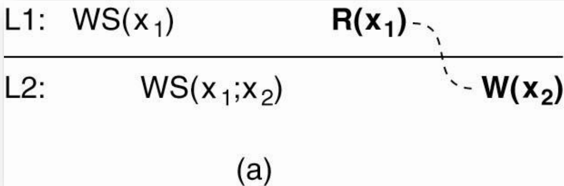
(a) A writes-follow-reads consistent data store
