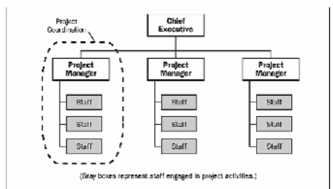
Figure 4.8: Project Organization
