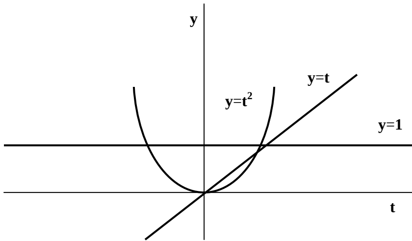
Figure 2 – The standard basis for P_2
