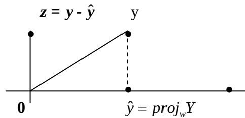
Fig: Orthogonal projection of y on to W .
