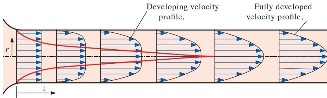
Fig. 1: The development of the velocity profile in a circular pipe.
