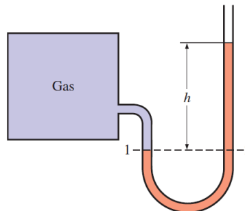
Figure: The basic manometer.
