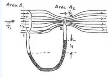
Figure 28.8: Venturi Meter
