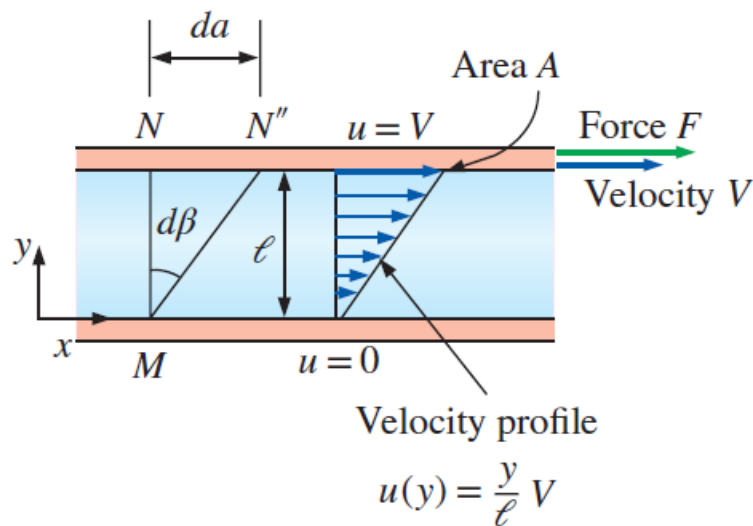
Fig. 1: The behavior of a fluid in laminar flow between two parallel plates when the upper plate moves with a constant velocity.
