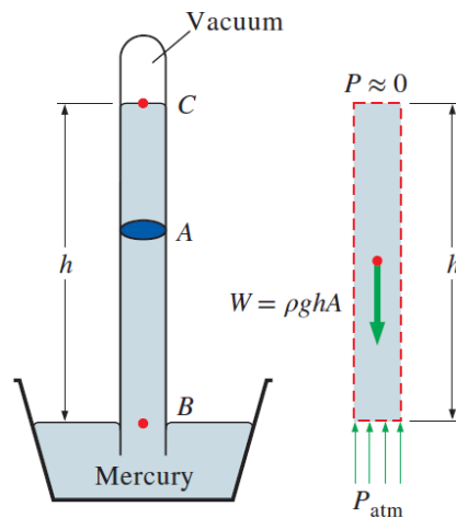
Figure: The basic barometer .
