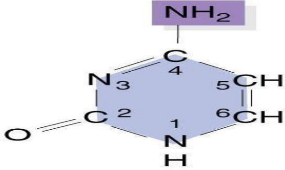
Cytosine (C)
