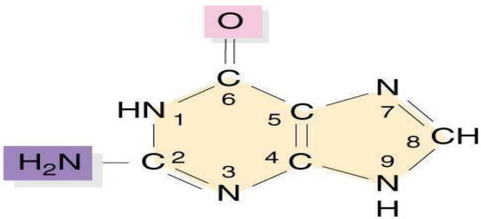
Guanine (G)
