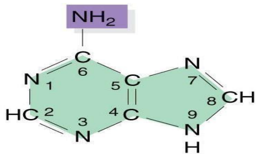
Adenine (A)
