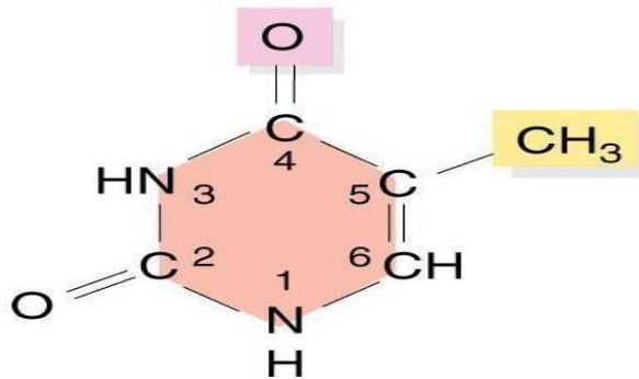
Thymine (T)
