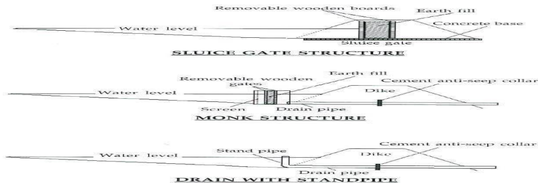
Figure 15: Cross sections of three structures used for draining ponds.
