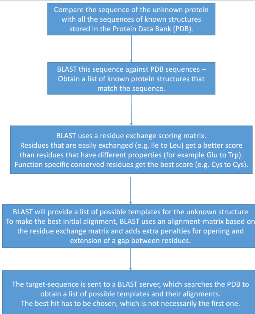
Figure 41.2.2: Working on selection of template &amp; target
