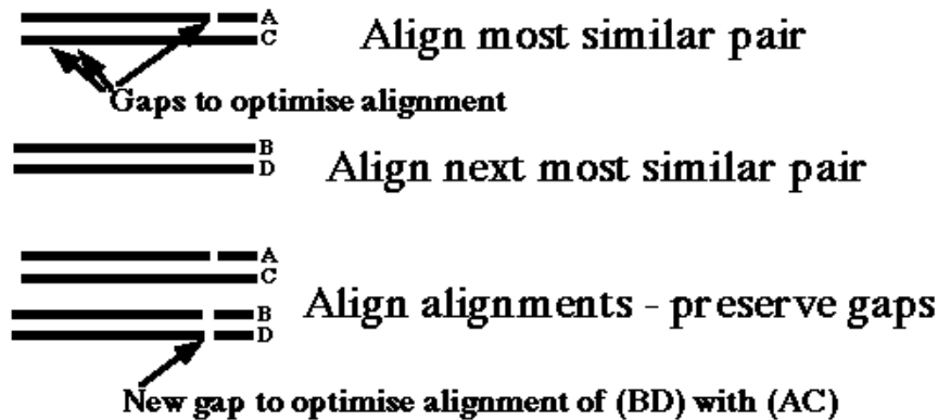
Figure 12.1.2: Progressive alignment
