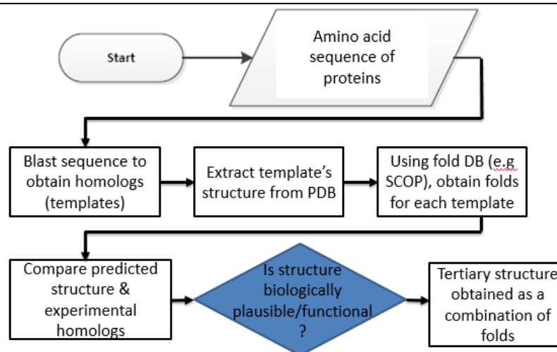
Figure 44.2.3: Flow chart of threading
