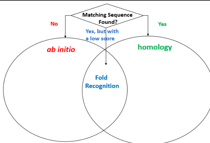
Figure 43.2.1: Comparative analysis of three different modelling techniques
