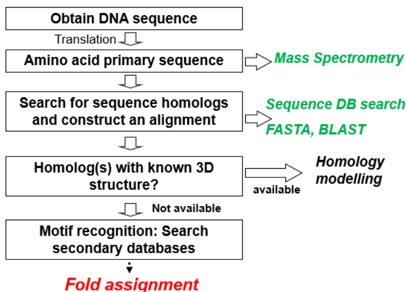
Figure 44.2.2: Initial steps before structural modelling
