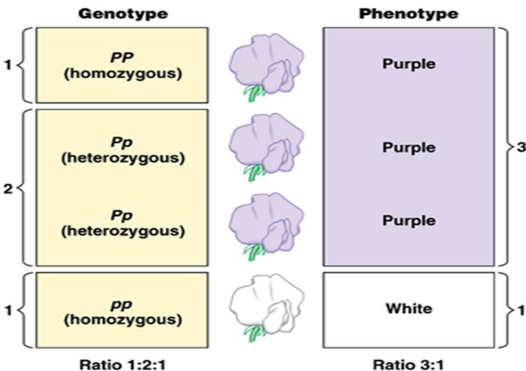
Figure 11.1 Genotype & Phenotype
