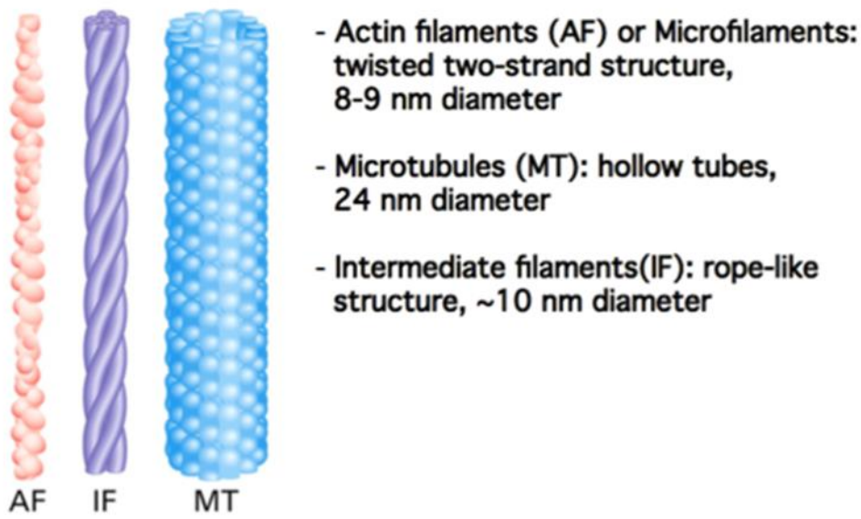
Figure 7.1 Cytoskeletal fibers
