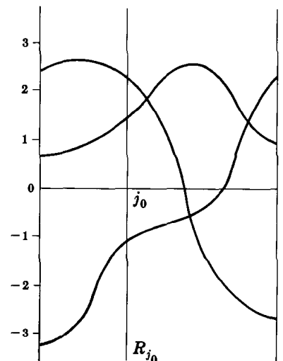
Members of X
