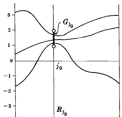
Members of \pi_{j_0}^{-1}[G_{j_0}]
