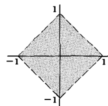
S_{d_2}(p, \delta) is shaded
