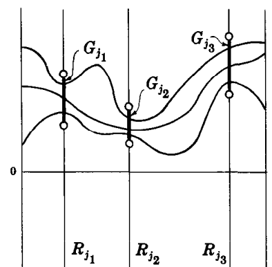
Members of B
