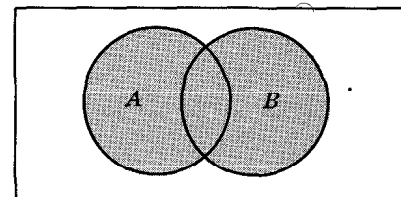
A \cup B is shaded
