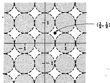
\mathcal{B} is displayed
