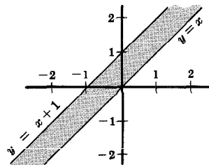
Graph of T^{-1}
